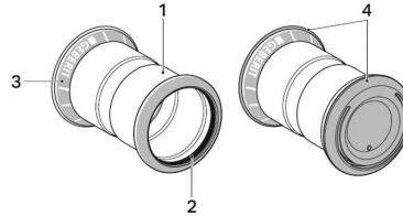
Figure 1: Structure of Geberit Mapress pressfitting
