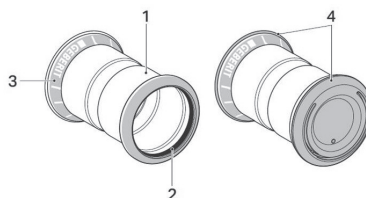
Figure 1: Structure of Geberit Mapress pressfitting
